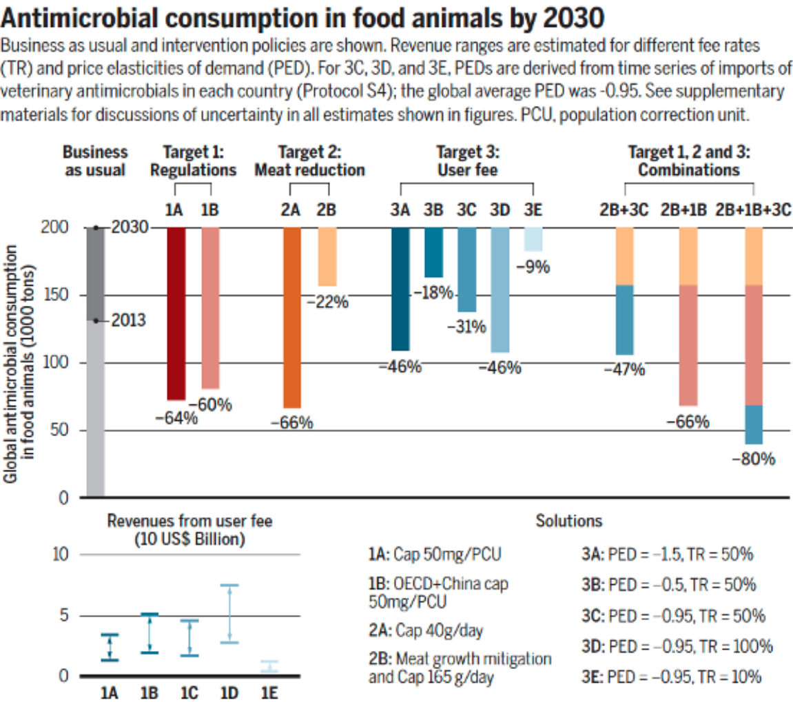
Figure 9. Antimicrobial consumption in food animals by 2030 Source: Van Boeckel, T. P. et al. Reducing antimicrobial use in food animals. Sci. Mag. 1350–1352 (2017). doi:10.1126/science.aaa1495
